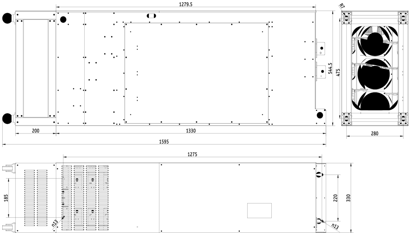
Dimensional drawing V900 - 315kW 4T3150
